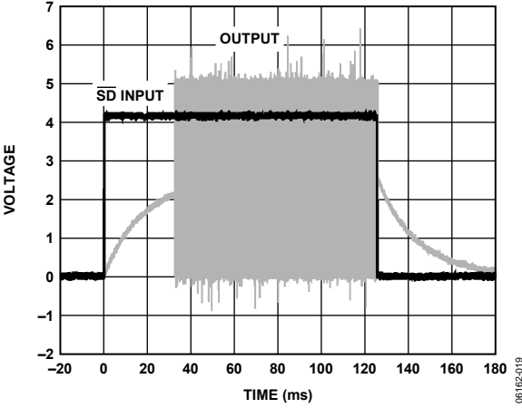
Figure 36. Turn-Off Response
